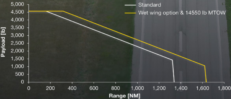
PAYLOAD-RANGE-DIAGRAM
